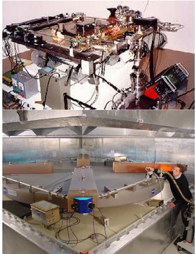
Figure 31. Ring laser gyroscope for Earth rotation monitoring. The picture shows the C-I (upper) ring laser installed in Canterbury, New Zealand, and the G ring laser at Wettzell, Germany (lower picture). From http://www.phys.canterbury.ac.nz/research/laser/pictures.-shtml .
