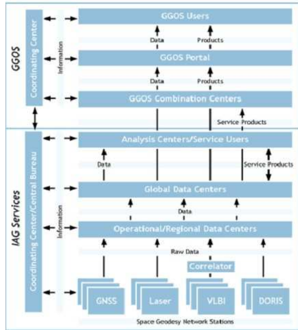
Figure 73. Each of the geometric IAG Services operates with a similar component structure for data flow and archive. The service-specific global data centers will provide data and products to the GGOS combination centers; GGOS users will obtain data and products through the GGOS Portal or through direct access to the service data centers. GGOS products will be accessible to users directly through the combination centers or through the GGOS portal.
