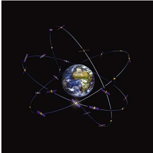
Figure 18. Artist's impression of the complete Galileo constellation of thirty satellites orbiting in three planes. The three MEO planes are at an inclination of 56^\circ with respect to the equatorial planes, resulting in a good coverage up to a latitude of 75^\circ . From http://esamultimedia.esa.int/images/navigation/ .
