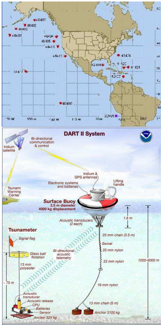
Figure 49. NOAA's DART stations. Top: Location of NOAA's DART stations. Bottom: Schematic illustration of the DART system. For explanation, see text. Figures taken from NOAA's DART system page at http://www.ndbc.noaa.gov/Dart/dart.shtml .
