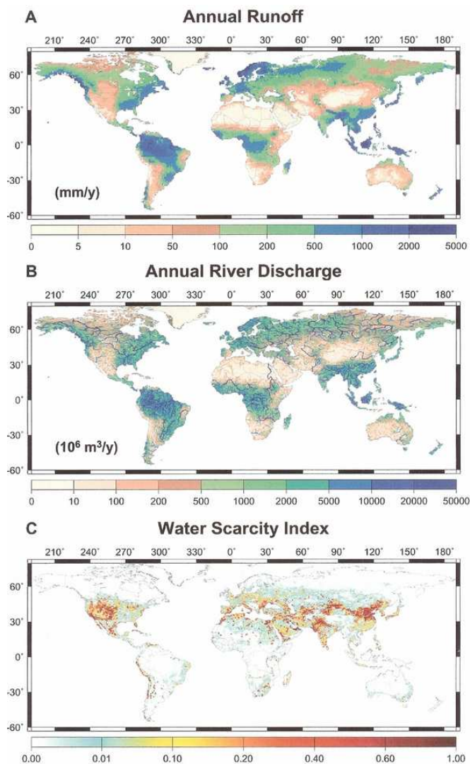
Figure 66. Earth's water resources: relation of supplies to demands. From Oki & Kanae (2006).
