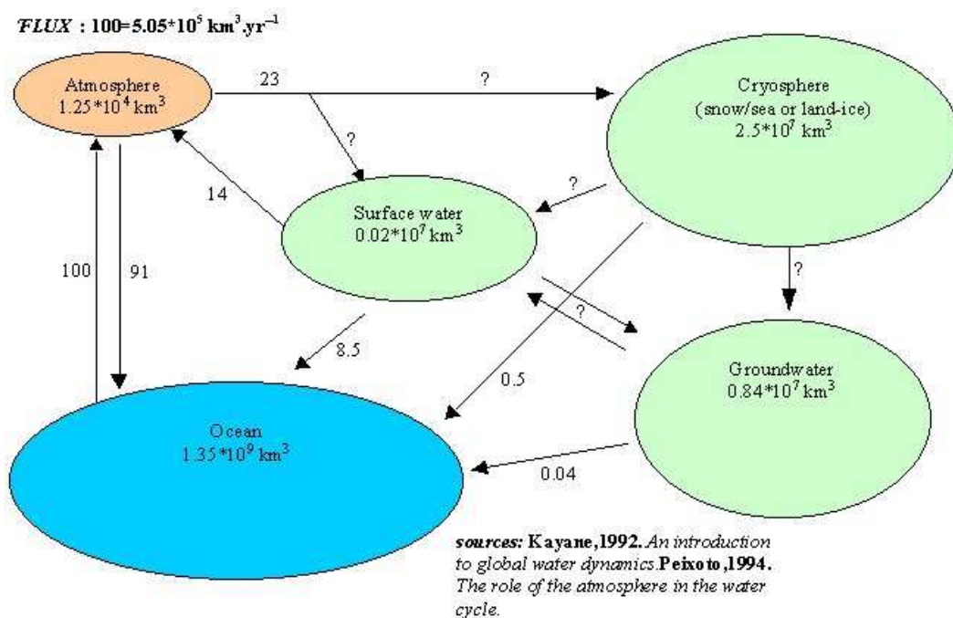
Global hydrological cycle and waterbalance. (Ovals are reservoirs, arrows are fluxes)
