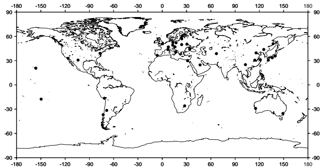
Figure 13. Tracking network of the ILRS.
