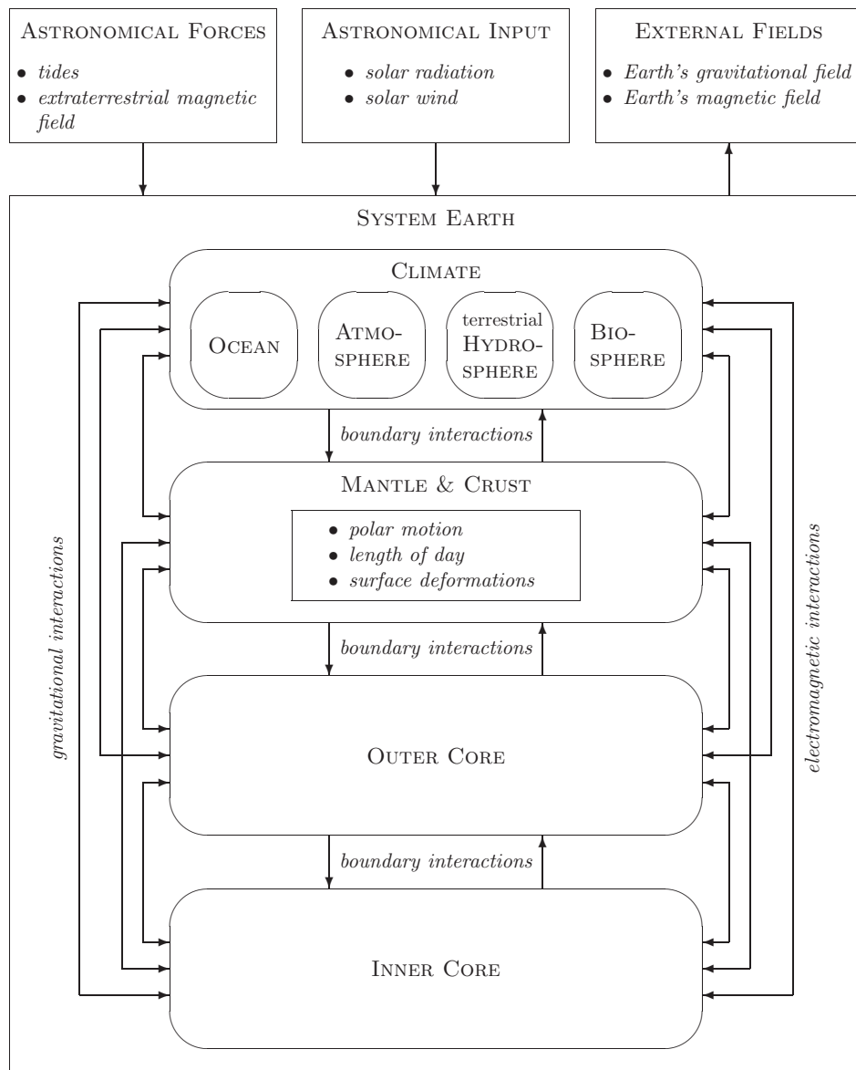
Figure 68. Components of the Earth system and their mechanical interactions. From Plag (2006a).
