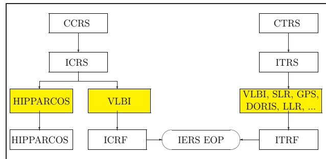
Figure 4. Overview of current conventional reference systems and their realizations. The current Conventional Celestial Reference Systems (CCRS) adopted by the IAU is the International Celestial Reference System (ICRS). In the radio-wavelength, this system is realized as ICRF through VLBI measurements of extragalactical objects and as such maintained by the IERS. At optical wavelengths, the observations made with the HIPPARCOS satellite allowed the materialization of the ICRS through the HIPPARCOS stellar frame. The tie between the HIPPARCOS and the ICRS is determined to a high degree of accuracy (Kovalevsky, 1997). The current Conventional Terrestrial Reference Systems (CTRS) accepted by IUGG is the International Terrestrial Reference System (ITRS), which is realized through the International Terrestrial Reference Frames (ITRF) maintained by the IERS. The tie between the ICRF and ITRF is provided by the IERS Earth Orientation Parameters (EOP). These describe the orientation of the Celestial Ephemeris Pole (CEP) in the terrestrial and celestial systems through the polar coordinates x and y and the nutation offsets d\psi and d\epsilon , respectively, and the orientation of the Earth around this axis through UT1-TAI as function of time. From Plag (2006a).
