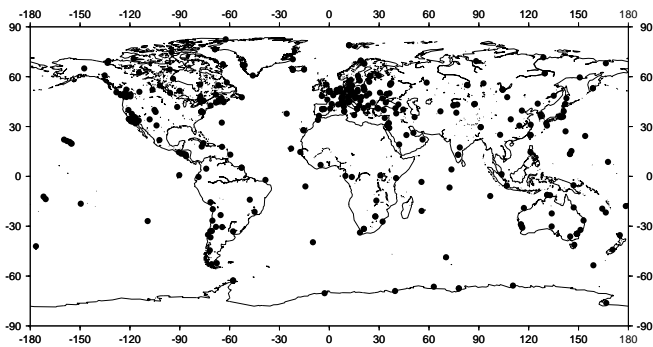
Figure 19. Tracking network of the IGS as of December 2006.
