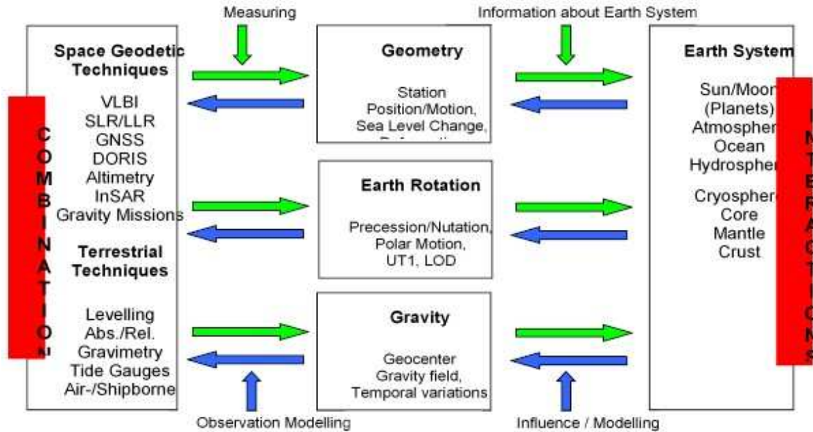
Figure 50. Measuring and modeling the Earth system.
