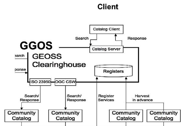
Figure 75. GGOS Clearinghouse architecture - engineering viewpoint (according to D. Nebert). Here, the term clearinghouse is used in its modern meaning of a search-able registry, i.e., a set of catalogs.
