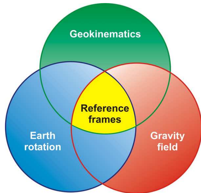
Figure 1. Constituents of an integrated geodetic monitoring system. The "three pillars" of geodesy provide the conceptual and observational basis for the reference frames required for Earth observation. Moreover, these three pillars are intrinsically linked to each other as they provide different observation of the same Earth system processes.
