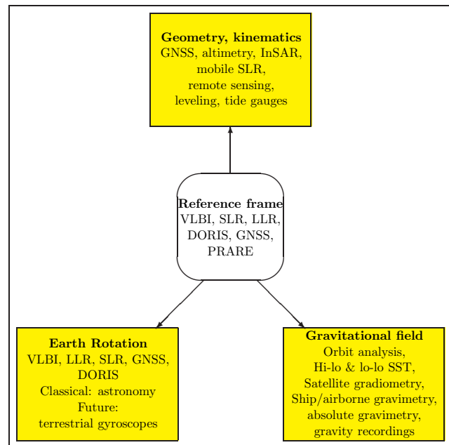
Figure 6. The three pillars of geodesy and their techniques. Today, the space-geodetic techniques and dedicated satellite missions are crucial in the determination and monitoring of geokinematics, Earth’s rotation and the gravity field. Together, these observations provide the basis to determine the geodetic reference frames with high accuracy, spatial resolution and temporal stability. From Plag (2006a), modified from Rummel (2000). For a list of acronyms, see Appendix C.
