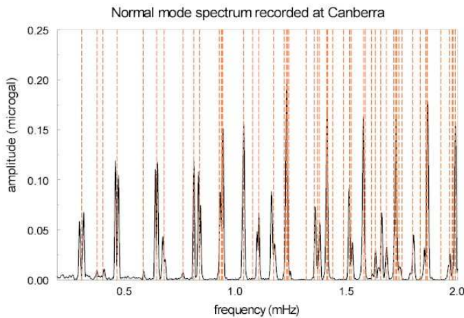
Figure 32. Long period normal modes from the Mw = 9.1 Sumatra-Andamen earthquake (2004/12/26) recorded by the SG at Canberra. The vertical lines are the theoretical multiplet peaks. The high signal-to-noise ratio is generally high.
