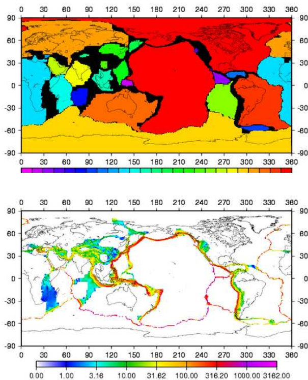
Figure 51. Model of tectonic plates. The model of the stable parts of the tectonic plates (top) is derived from the strain field (bottom) (Kreemer et al., 2003). The upper diagram shows the individual stable parts of the plates by different colors. For large areas, the surface is deforming and the exact location of the plate boundaries is often uncertain.
