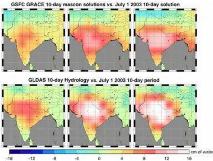
Figure 39. GRACE-determined variations in water storage on land. Upper row: Ten-day estimates of the mass change with respect to a multi-year averaged gravity model in a 4^\circ \times 4^\circ grid. The values shown are the mass change mapped into an equivalent change in a surface layer of water in units of cm. To estimate these values, the effects of atmospheric pressure changes and solid Earth and ocean tides have been removed based on model predictions. Lower row: Numerically modeled soil moisture and snow mass fields from the Global Land Data Assimilation System (GLDAS) by Rodell et al. (2004). From http://grace.sgt-inc.com/ .
