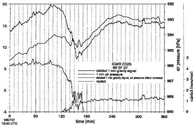
Figure 33. Example of atmospheric mass transport during heavy rain. The signal at the top of the figure (at the start of the record) is gravity with tides removed, and the curve beside it is the pressure. After correcting with a frequency dependent admittance, the residual gravity is the lower curve (left). Note this residual gravity begins to decrease sharply just before the onset of the rain (lowest curve) due to a mass increase above the station that is not seen in the surface pressure.
