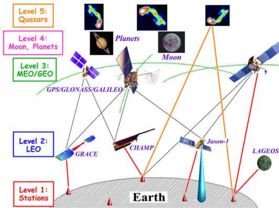
Figure 70. The five levels of GGOS and their interactions with observations of various types. The combined infrastructure allows the determination and maintenance of the global geodetic reference frames, and the determination of Earth's gravity field and rotation. The ground networks and GNSS are crucial in positioning. In particular, they allow the monitoring of volcanoes, earthquakes, tectonically active regions and landslide-prone areas. The LEO satellites monitor sea level, ice sheets, water storage on land, atmospheric water content, high-resolution surface motion, and variations in the Earth's gravity field. The latter are caused, to a large extent, by regional and global transport in the hydrological cycle.
