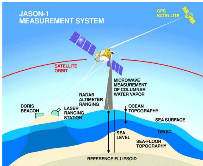
Figure 25. The Jason-1 satellite altimetry mission. Courtesy NASA/JPL.
