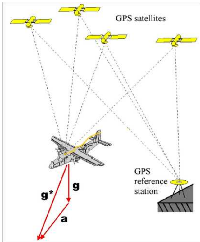
Figure 36. Principle of airborne gravimetry.
