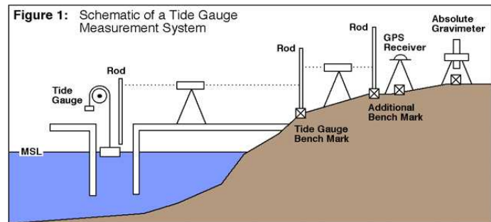
Figure 47. Principle of tide gauge measurements. From http://sealevel.colorado.edu/tidegauges.html . See also IOC (2006).
