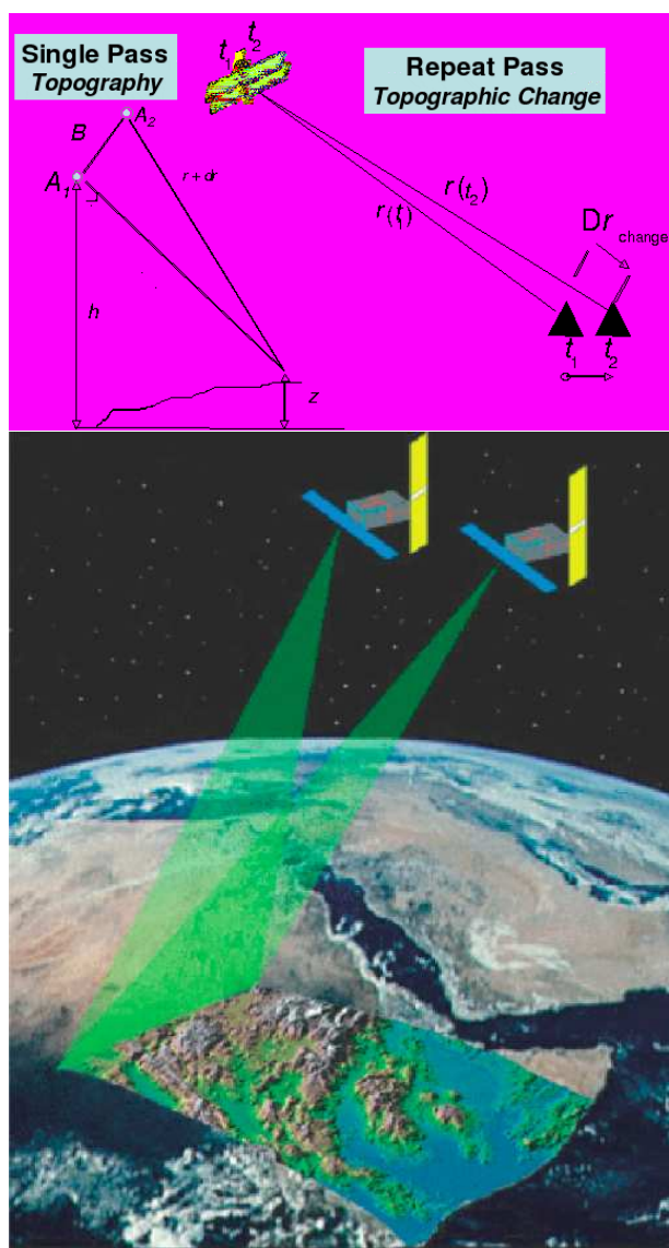
Figure 29. Principle of InSAR. Two antenna separated in space can be used to determine topography (top), while an exact repeat pass of a radar instrument can be used to determine topographic or surface change (bottom).
