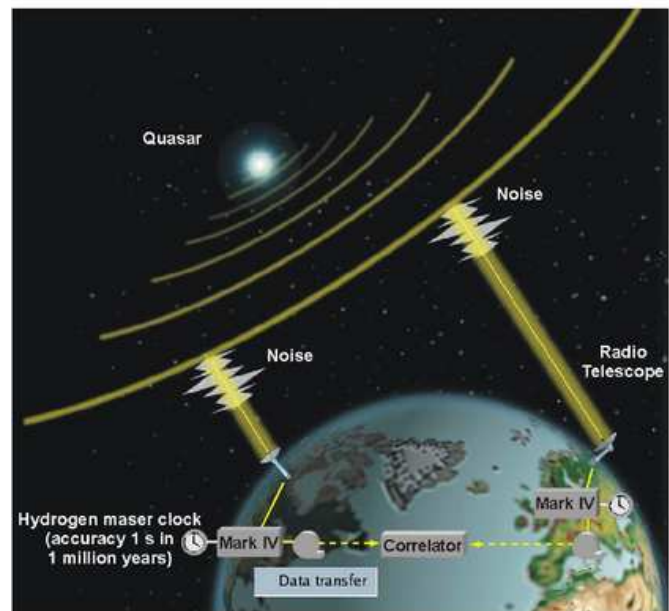
Figure 8. Principle of very long baseline interferometry.
