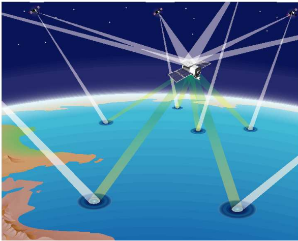
Figure 27. Use of reflected GNSS signals for altimetric measurements. An Earth-orbiting instrument uses direct GNSS signals for precise positioning, but also receives reflected signals to make several simultaneous bistatic altimetric measurements.
