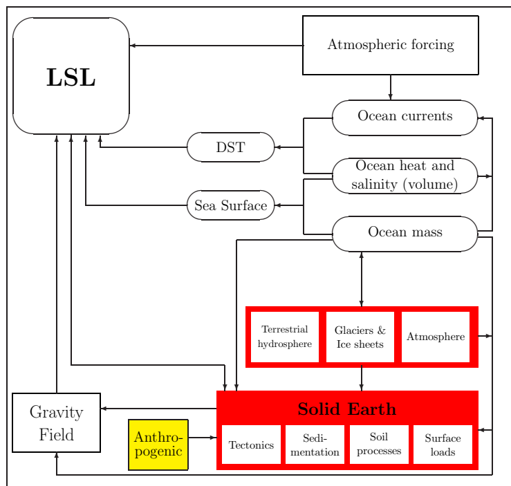
Figure 63. Processes and factors affecting long-period local sea level. Mass movements in the terrestrial hydrosphere (groundwater, rivers, lakes, and reservoirs) and land-based cryosphere (glaciers and ice sheets) and mass exchange with the ocean load and deform the solid Earth and affect the gravity field. The deformations and the associated gravitational changes result in LSL changes, depending on where mass has been relocated. Ocean mass changes as well as ocean volume changes caused by heat and salinity changes affect the sea surface position. Heat and salinity changes also affect the ocean currents and thus change the Dynamic Sea Surface Topography (DST). Atmospheric circulation forces regional wind-driven currents affecting the DST. DST and sea surface changes caused by regional and global processes change LSL in any location. The atmosphere also acts locally on the sea surface and thus changes sea level. Past changes in the ice sheets and glaciers lead to postglacial rebound, which affects sea level through vertical land motion and geoid changes. Tectonic processes in the solid Earth both result in vertical land motion, changes in the size of the ocean basins, and changes in the geoid. In areas where sedimentation takes place, the compaction of the sediments and their load on the solid Earth intro-
