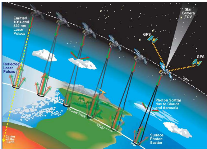
Figure 24. Principle of satellite altimetry. From http://icesat.gsfc.nasa.gov .
