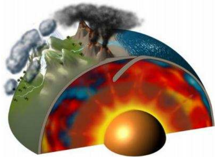
Figure 3. The dynamic Earth. The interaction of solid Earth, hydrosphere, and atmosphere processes has created a highly complex system. From Solomon & the Solid Earth Science Working Group (2002).
