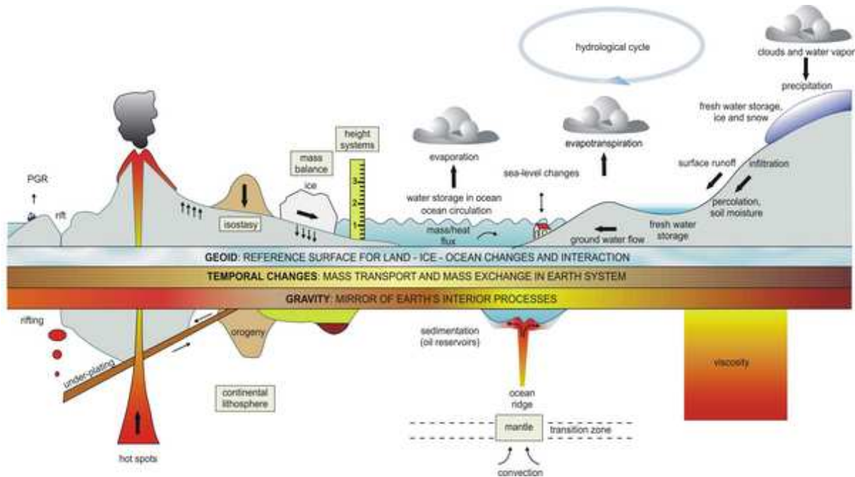
Figure 52. The interrelation of gravity, gravity variations, mass transport and distribution.
