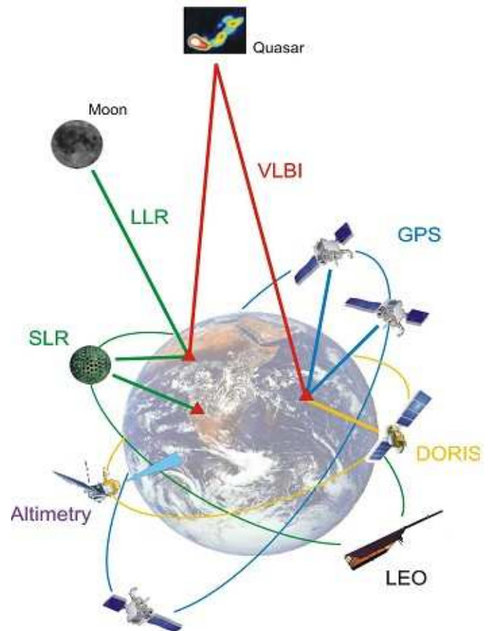
Figure 76. Combination and integration of the geodetic observation techniques. The combined infrastructure allows the determination and maintenance of the global geodetic reference frames, and the determination of Earth's gravity field and rotation. The ground networks and navigation satellites (currently in particular GPS) are crucial in positioning, with applications to all SBAs. In particular, they allow the monitoring of volcanoes, earthquakes, tectonically active regions and landslide-prone areas. The Low Earth Orbit (LEO) satellites monitor sea level, ice sheets, water storage on land, atmospheric water content, high-resolution surface motion, and variations in the Earth's gravity field. The latter are caused, to a large extent, by regional and global mass transport in the hydrological cycle.
