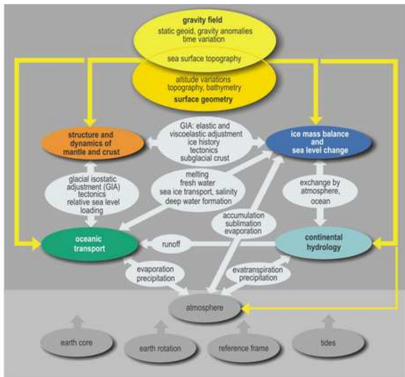
Figure 53. Interconnections between processes and research themes related to mass transport and mass distribution. Arrows in the center of the figure indicate mass exchange and dynamic feedback mechanisms. Other arrows connect the gravimetric and geometric observations (on top of the figure) to the physical processes or indicate external influences and complementary fields (at the bottom of the figure).
