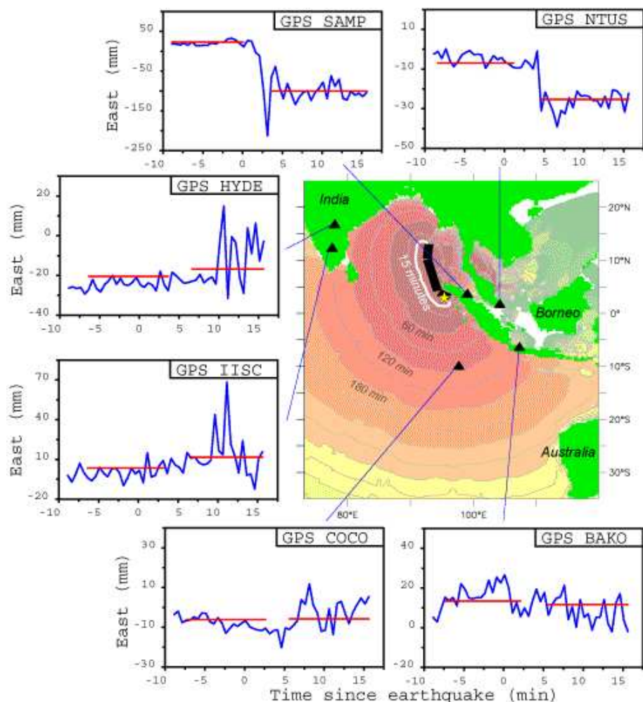
Figure 61. Seismic moment determination based on GNSS. Time series (blue lines) of east component of ground displacements after the great December 2004 Sumatra earthquake, recorded by continuous GPS sites in Southeast Asia. The earthquake produced changes in site positions that are large enough to allow the magnitude of the earthquake to be assessed within 15 minutes, faster than was possible with seismic data alone. This time interval is shorter than the time required by the tsunami to cross the Indian Ocean, illustrating that GNSS data can contribute to tsunami warning by assessing whether an earthquake is large enough to generate an oceanwide tsunami. The tsunami arrival times (color contours on map) are made available by NOAA Center for Tsunami Research (director: Dr. Frank Gonzalez). From Blewitt et al. (2006b)
