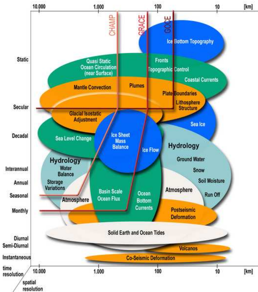
Figure 54. Resolvability of Mass transport by satellite missions. Mass transport phenomena and mass distribution characteristics and its resolvability by the satellite missions CHAMP, GRACE and GOCE.
