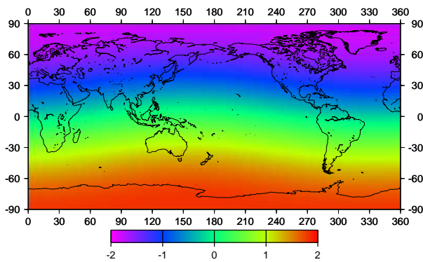
Figure 5. Effect of secular translation between ITRF2000 and ITRF2005 on vertical rates. The vertical rates are for a secular translation velocity of \vec{d} = (-0.2, 0.1, -1.8) mm/yr as given on http://itrf.ensg.ign.fr/ITRF_solutions/2005/ .
