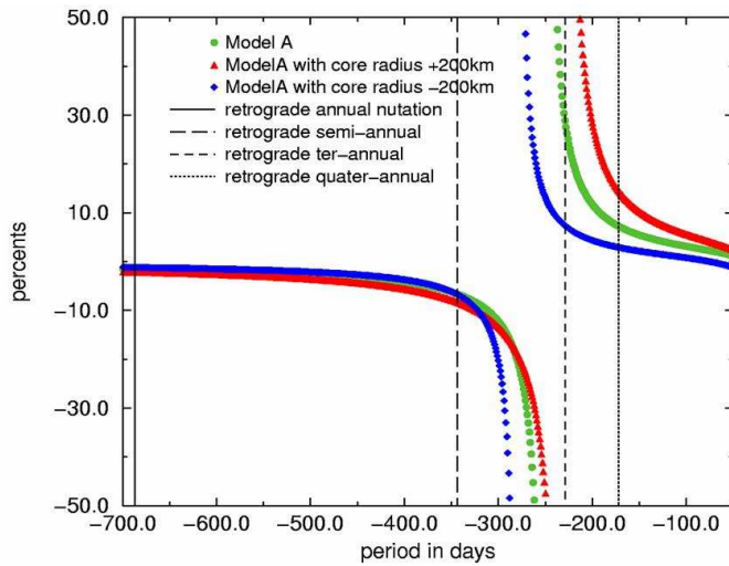
Figure 67. Resonance induced when different dimensions of the core are considered. The vertical lines show where nutation could be observed.
