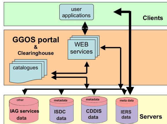
Figure 74. GGOS portal architecture.
