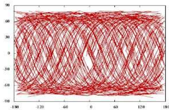
Figure 28. Reflection point loci for one receiver at 400 km, assuming its antenna beam can capture all available reflections, per day. Horizontal axis is longitude, vertical axis is latitude.
